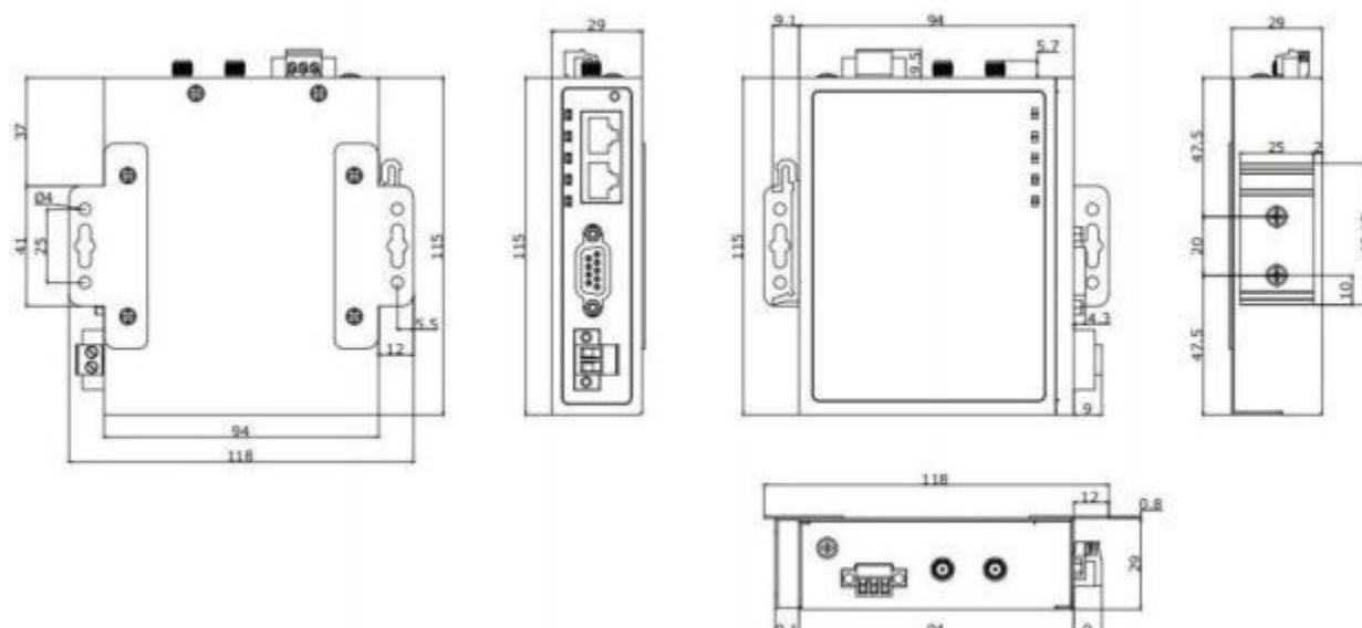
Fig.1 Dimension
