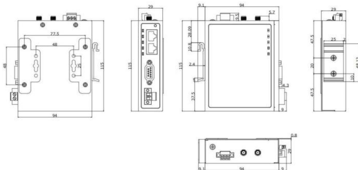
Fig.1 Dimension
