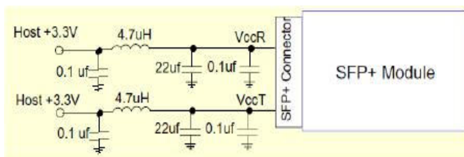
Recommended Host Board Power Supply Circuit
